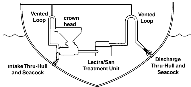
At or Below Waterline Installation Shown
