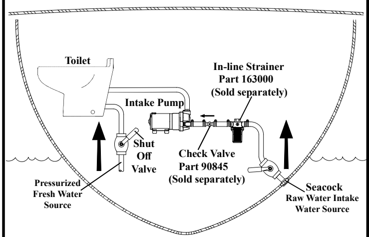
FIG 7 Sample Plumbing Diagram for Above Waterline Installations
