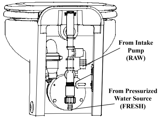
FIG 5 SeaEra QC Water Connections
