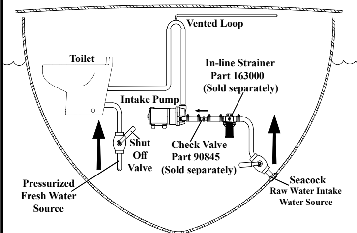
FIG 6 Sample Plumbing Diagram for Below Waterline Installations
