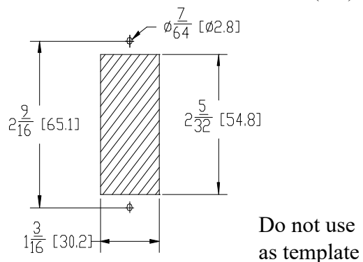
FIG 1 Selection Switch cutout sizes inches (mm)
