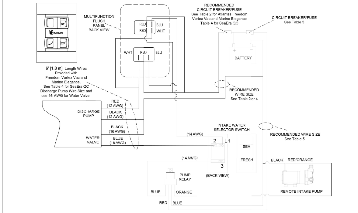
FIG 8 WIRING MULTIFUNCTION FLUSH PANEL TO SEA/FRESH MODEL
