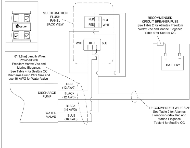
FIG 8 WIRING MULTIFUNCTION FLUSH PANEL TO SEA/FRESH MODEL
