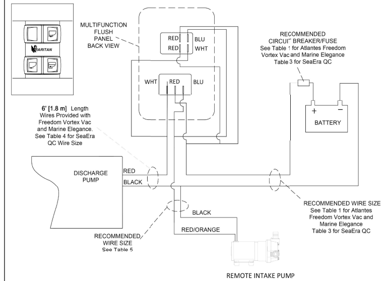
FIG 8 WIRING MULTIFUNCTION FLUSH PANEL TO SEA/FRESH MODEL
